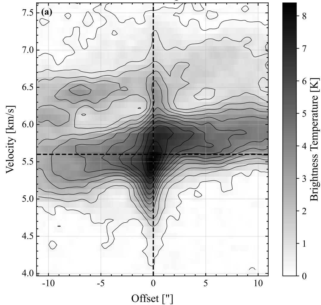
\text{C}^{18}\text{O} PV Diagram
